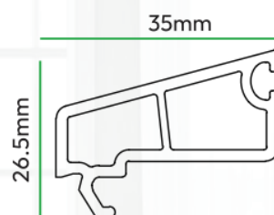
35x26.5mm casement single glass bead
