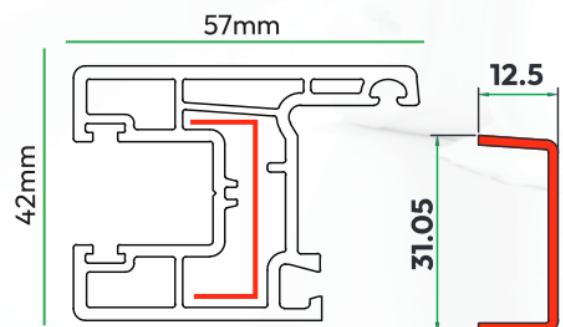
57x42mm sliding sash
