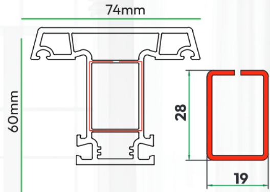
74x60mm casement mullion
