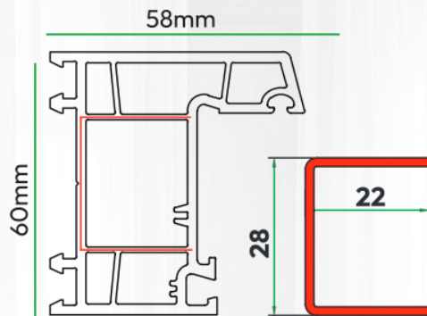
60x58mm casement frame
