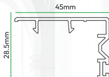
45x28.5mm sliding sash interlock
