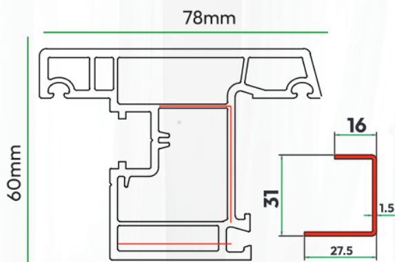
78x60mm outward window sash
