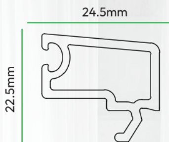
24.5x22.5mm sliding single glass bead
